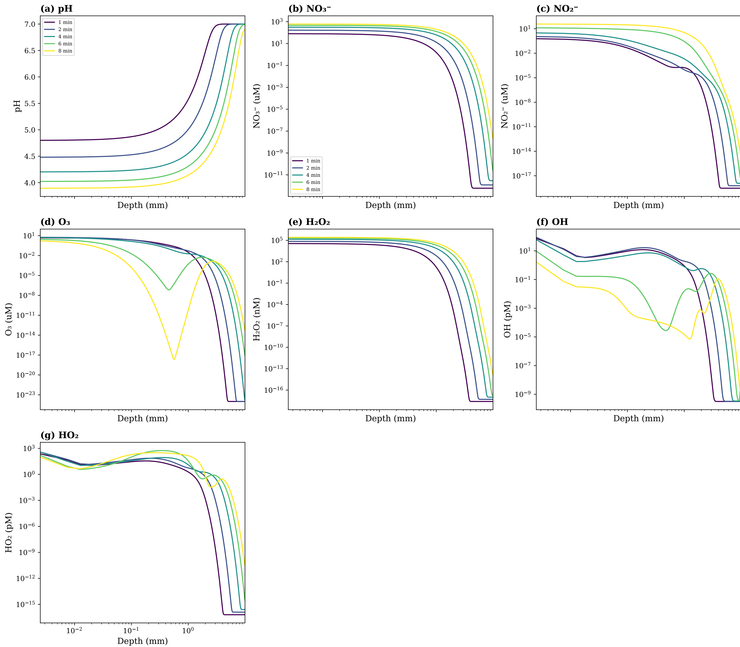
Spatial profiles (DIW, three_film, \delta g=10\text{mm} )
